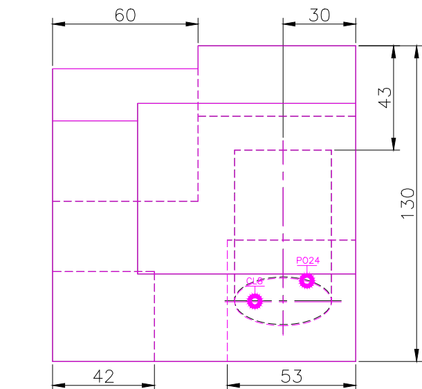
TOP SCALE 1/2
