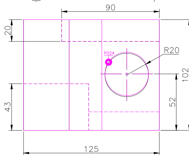
FRONT SCALE 1/2
