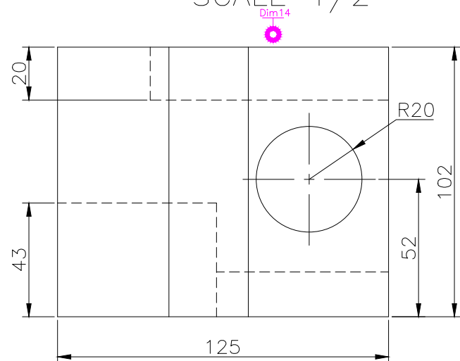
FRONT SCALE 1/2
