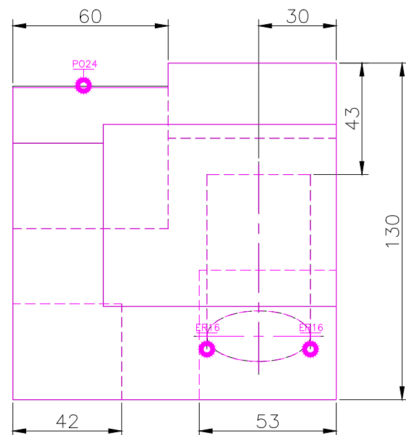
TOP SCALE 1/2
