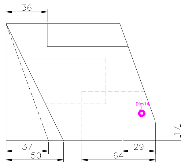
RIGHT SCALE 1/2
