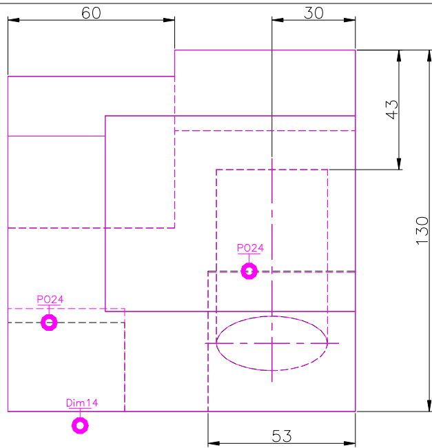
top SCALE 1/2
