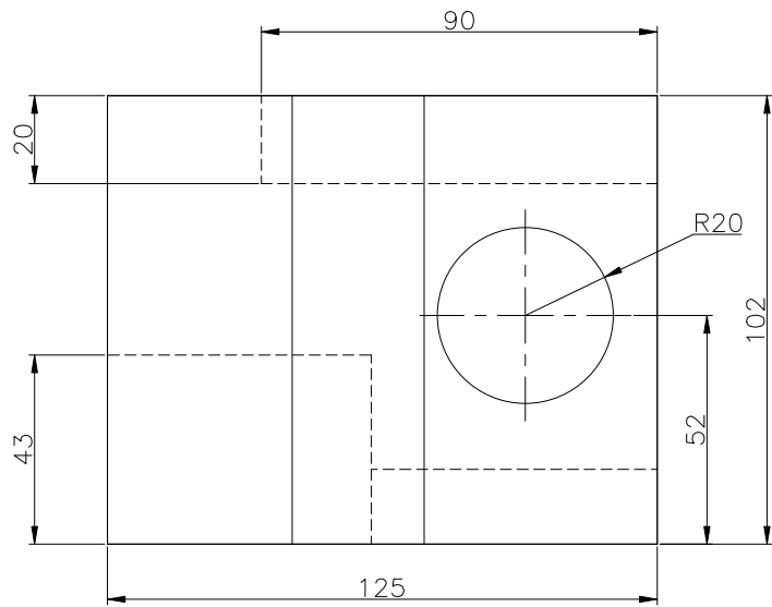
FRONT SCALE 1/2
