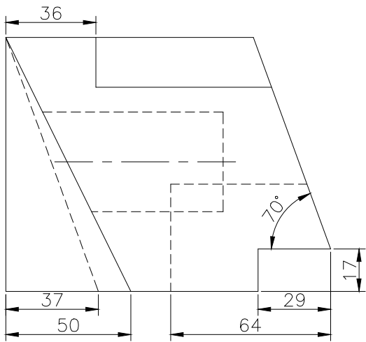
RIGHT SCALE 1/2
