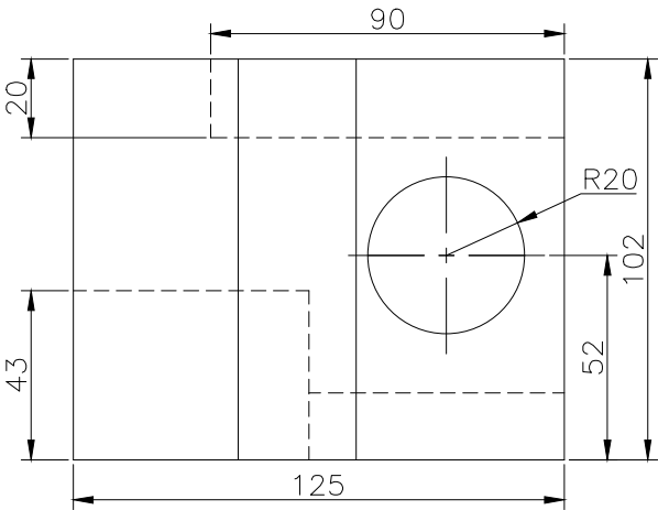
FRONT SCALE 1/2
