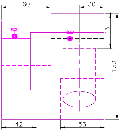
TOP SCALE 1/2
