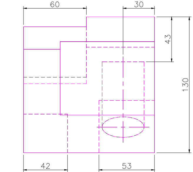
TOP SCALE 1/2
