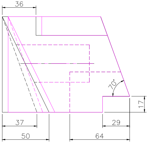
RIGHT SCALE 1/2
