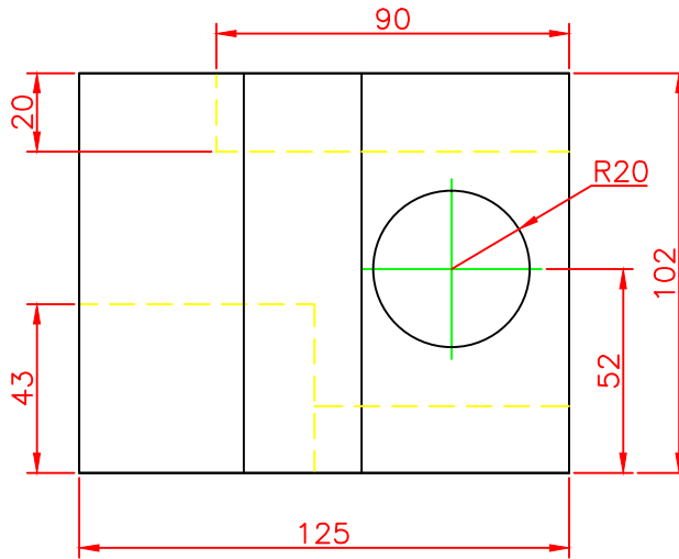
FRONT SCALE 1/2
