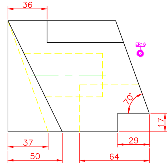
RIGHT SCALE 1/2
