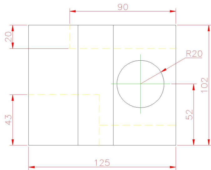
FRONT SCALE 1/2
