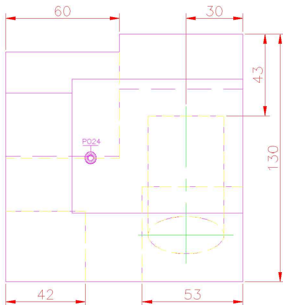
TOP SCALE 1/2
