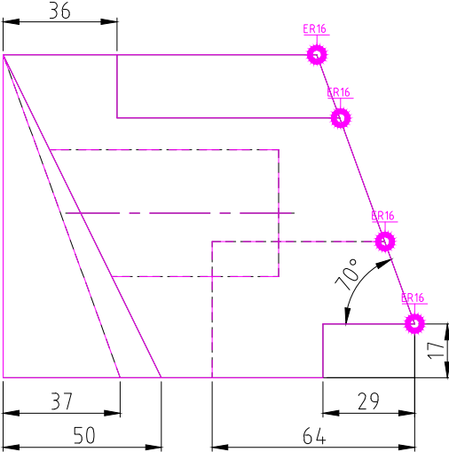
RIGHT SCALE 1/2
