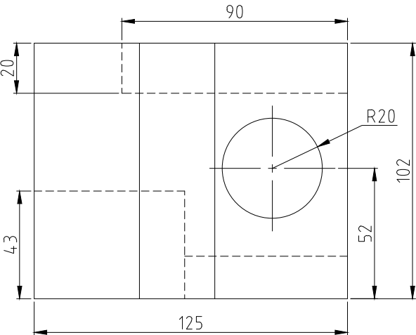
TOP SCALE 1/2
