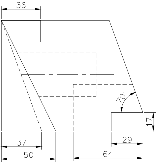
RIGHT SCALE 1/2
