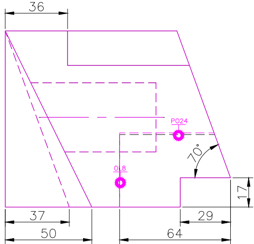
RIGHT SCALE 1/2
