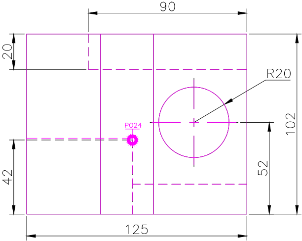
FRONT SCALE 1/2
