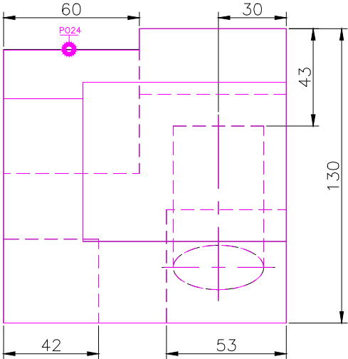
TOP SCALE 1/2
