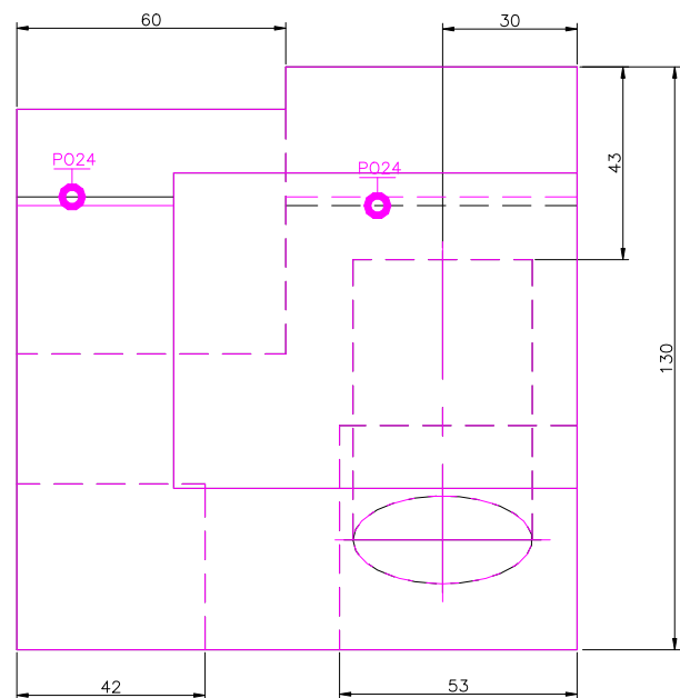
TOP SCALE 1/2
