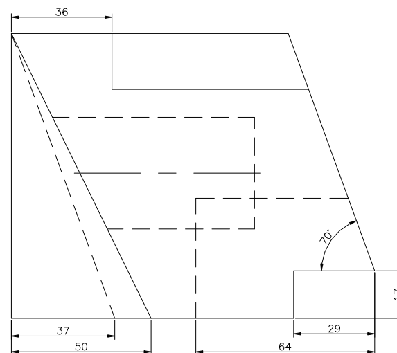
RIGHT SCALE 1/2
