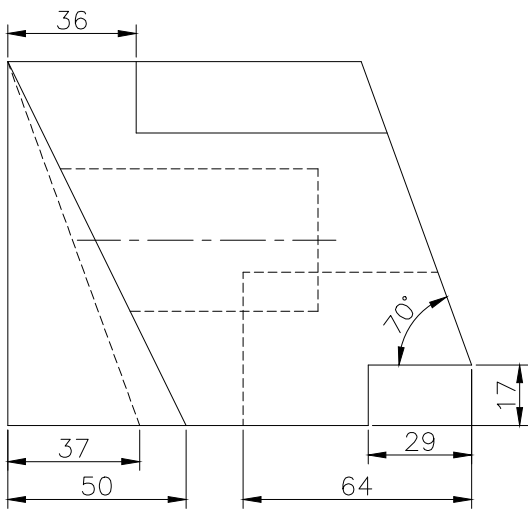
RIGHT SCALE 1/2
