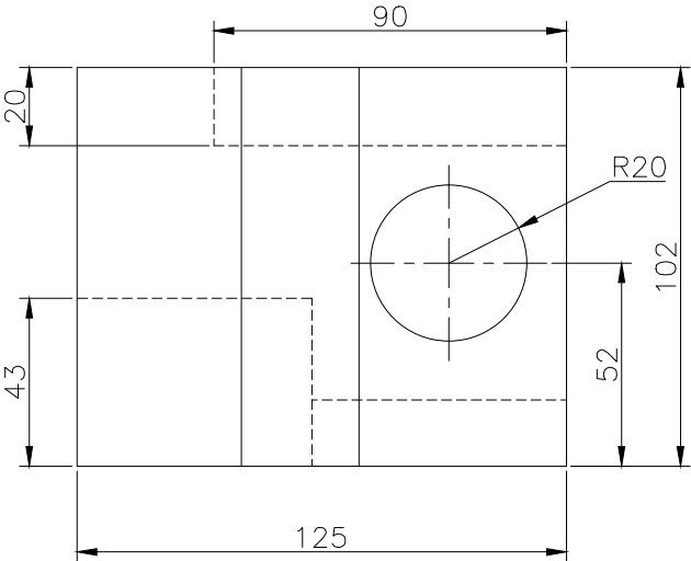
FRONT SCALE 1/2
