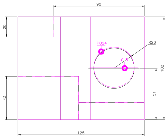
FRONT SCALE 1/2
