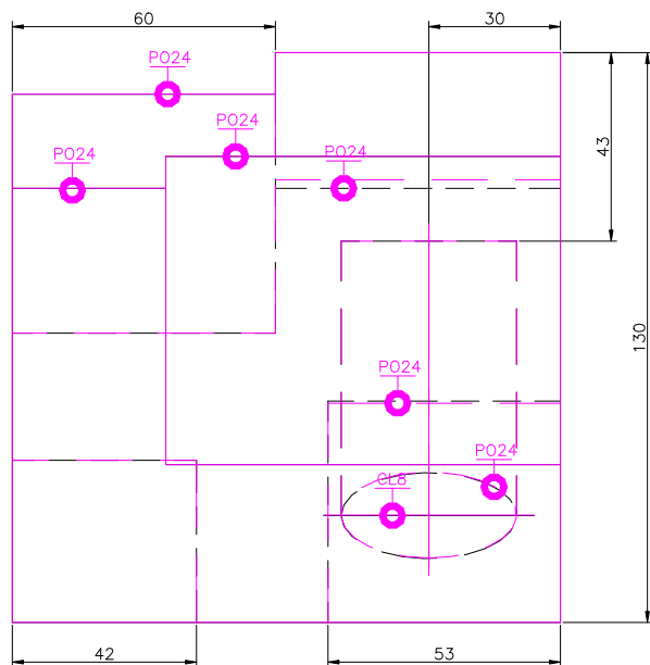
TOP SCALE 1/2
