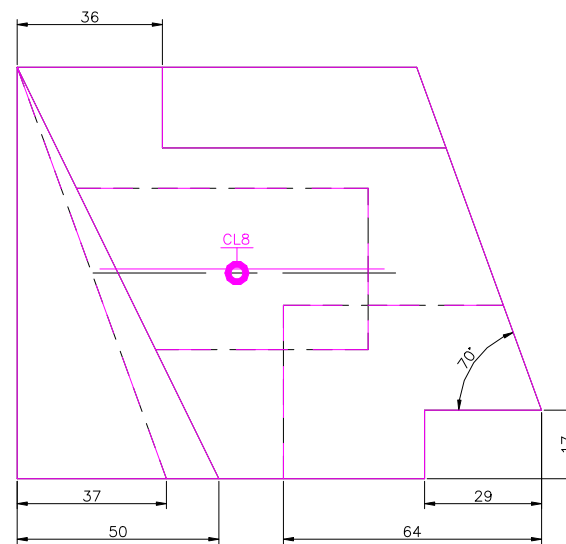
RIGHT SCALE 1/2
