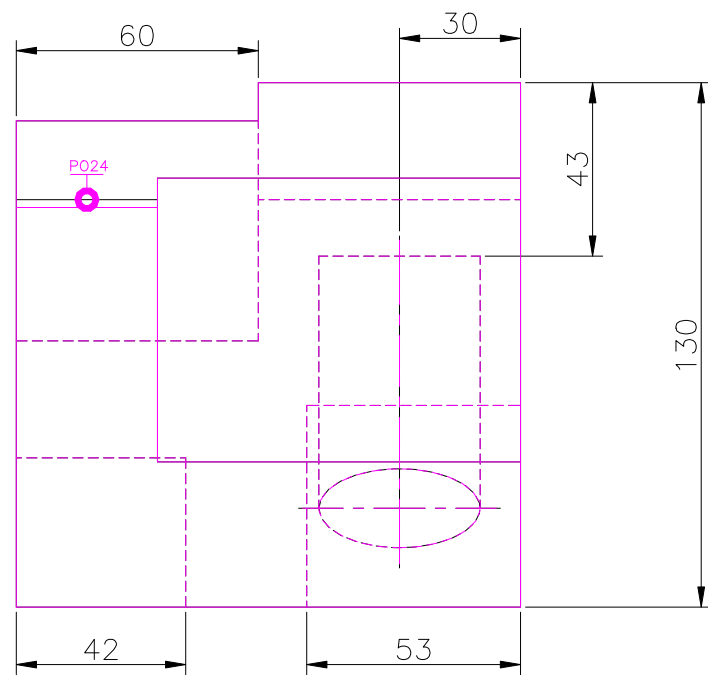
FRONT SCALE 1/2
