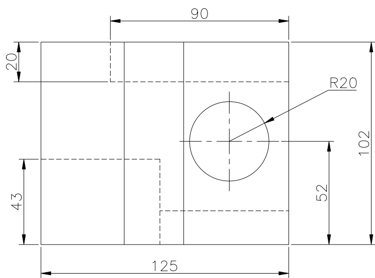
FRONT SCALE 1/2
