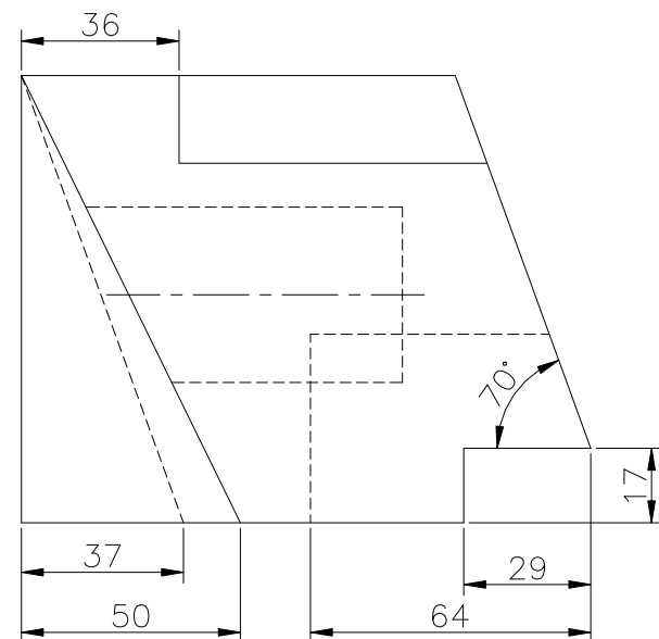
RIGHT SCALE 1/2
