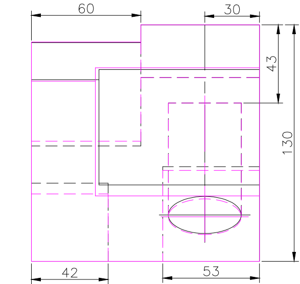
TOP SCALE 1/2
