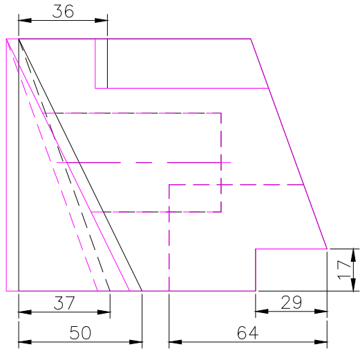
RIGHT SCALE 1/2
