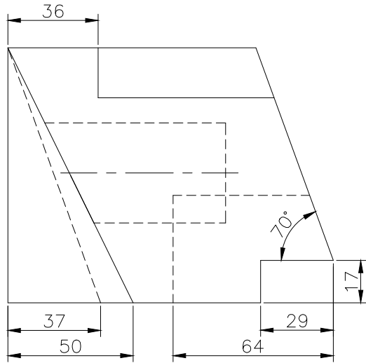
RIGHT SCALE 1/2
