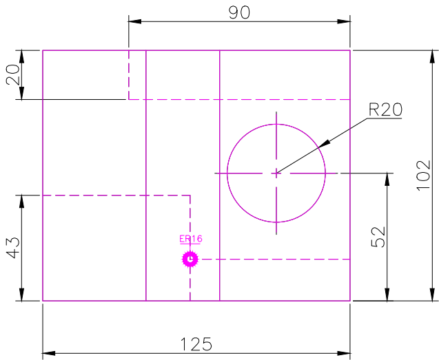
FRONT SCALE 1/2
