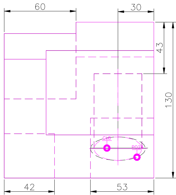
TOP SCALE 1/2
