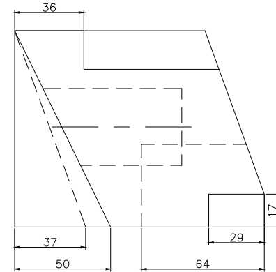
RIGHT SCALE 1/2
