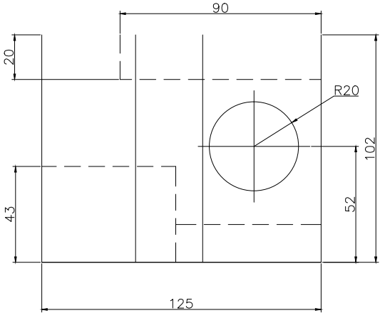
FRONT SCALE 1/2
