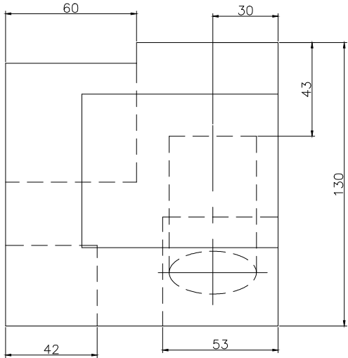
TOP SCALE 1/2
