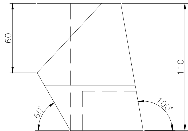
RIGHT SCALE 1/2
