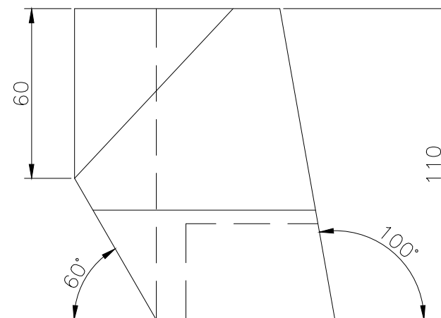
RIGHT SCALE 1/2
