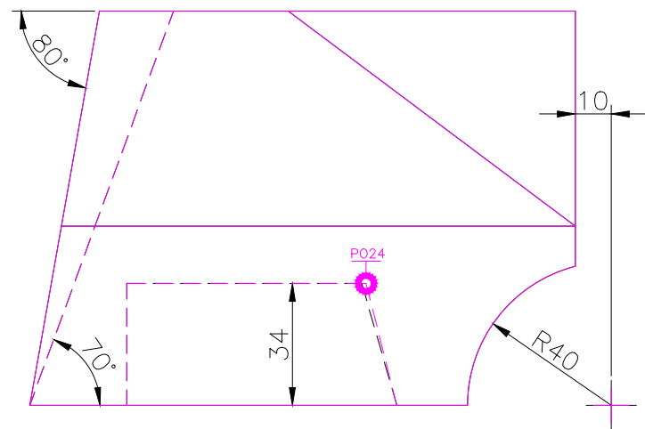
FRONT SCALE 1/2
