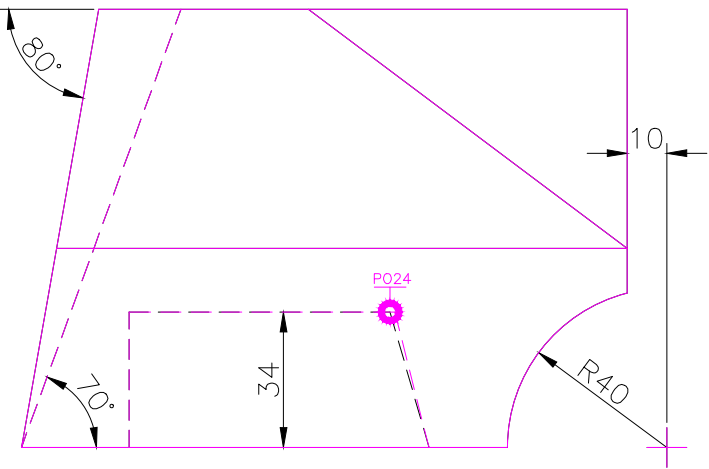
FRONT SCALE 1/2
