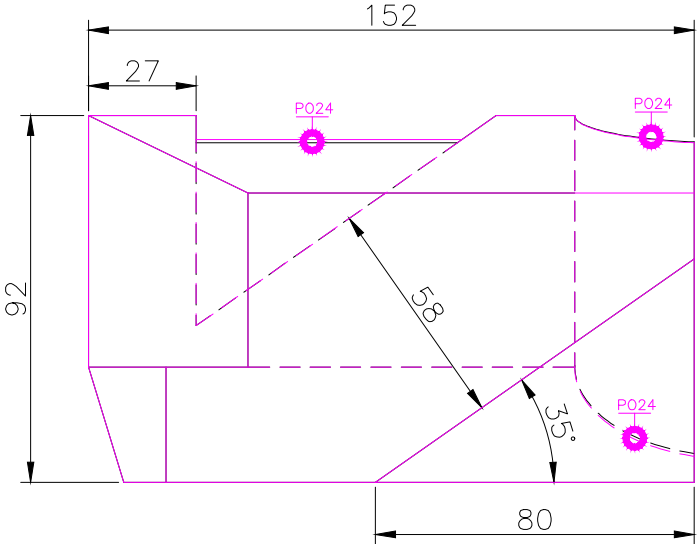
TOP SCALE 1/2
