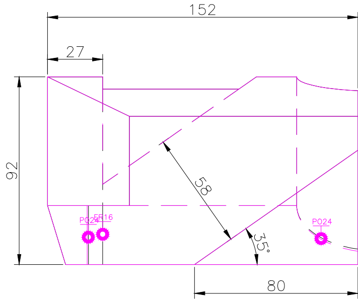
TOP SCALE 1/2
