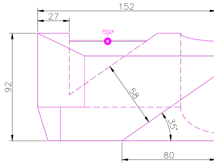
TOP SCALE 1/2
