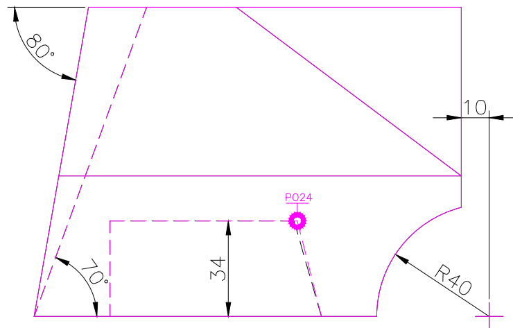
FRONT SCALE 1/2
