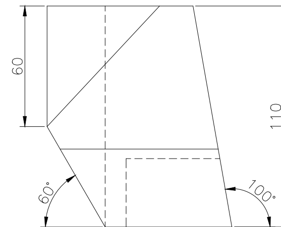
RIGHT SCALE 1/2
