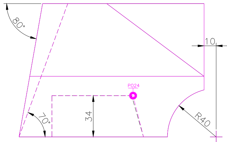
FRONT SCALE 1/2
