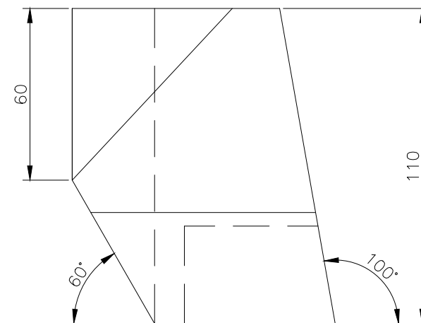
RIGHT SCALE 1/2
