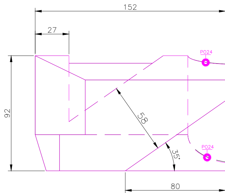
TOP SCALE 1/2
