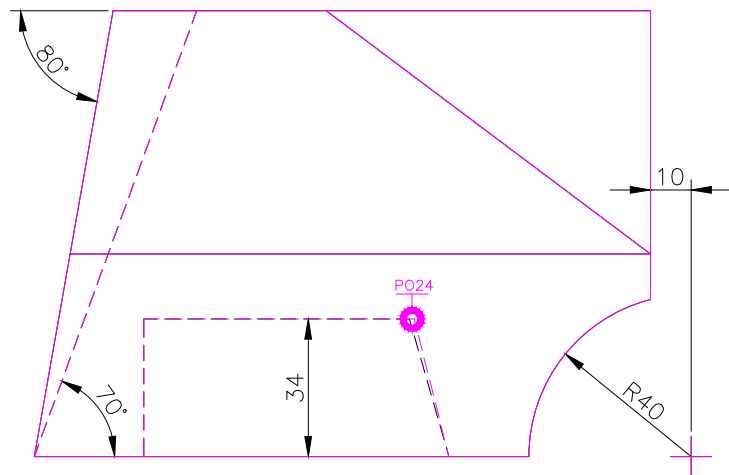
FRONT SCALE 1/2
