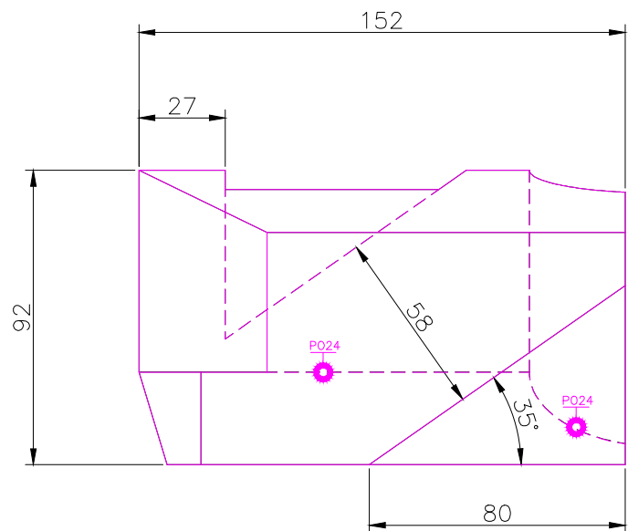
TOP SCALE 1/2
