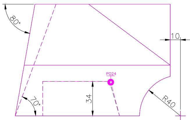
FRONT SCALE 1/2
