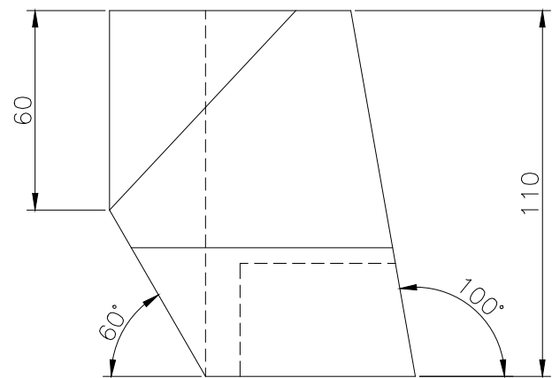
RIGHT SCALE 1/2
