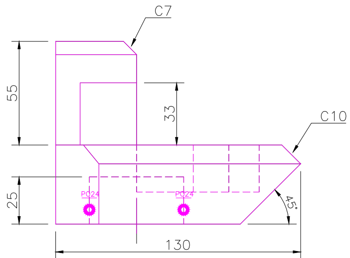
FRONT SCALE 1/2
