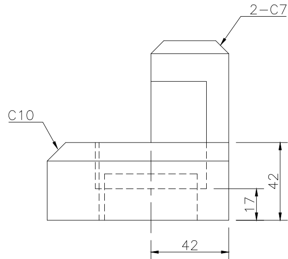
RIGHT SCALE 1/2
