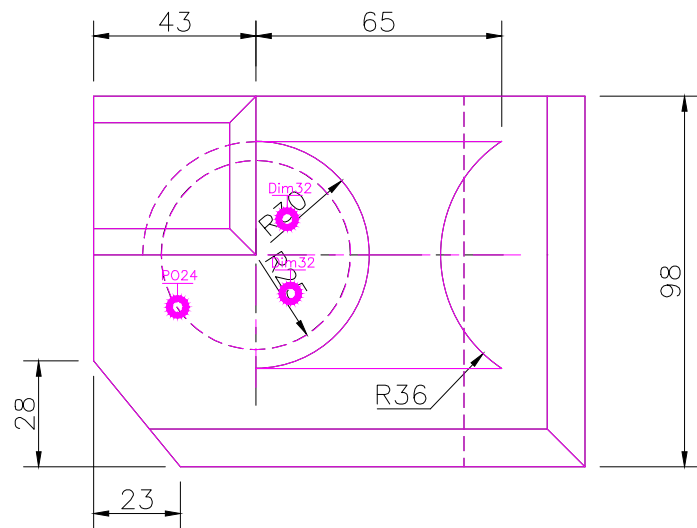
TOP SCALE 1/2
