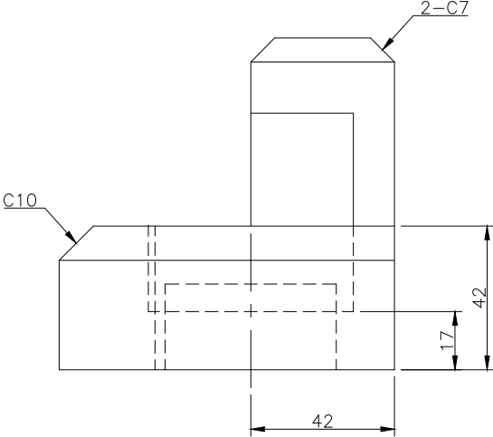
RIGHT SCALE 1/2
