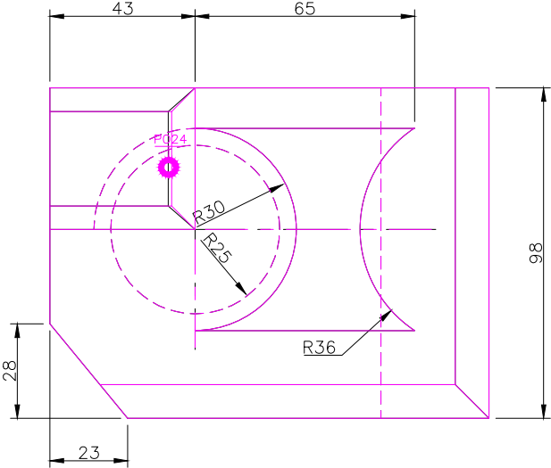
TOP SCALE 1/2
