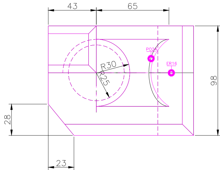
TOP SCALE 1/2
