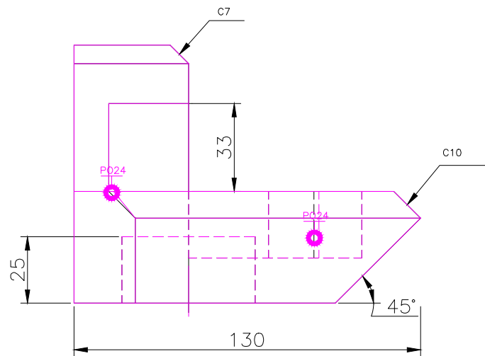
FRONT SCALE 1/2
