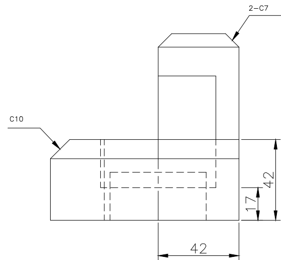
RIGHT SCALE 1/2
