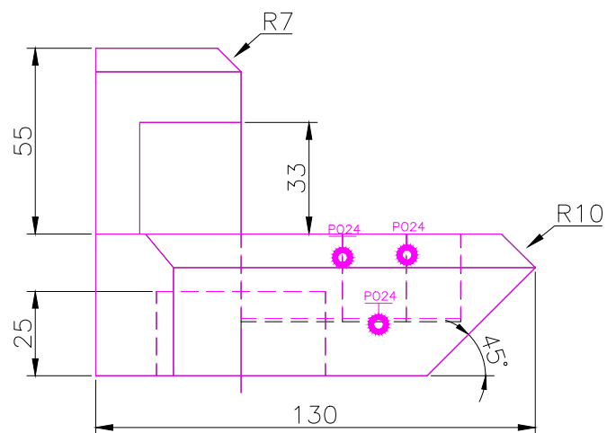
FRONT SCALE 1/2
