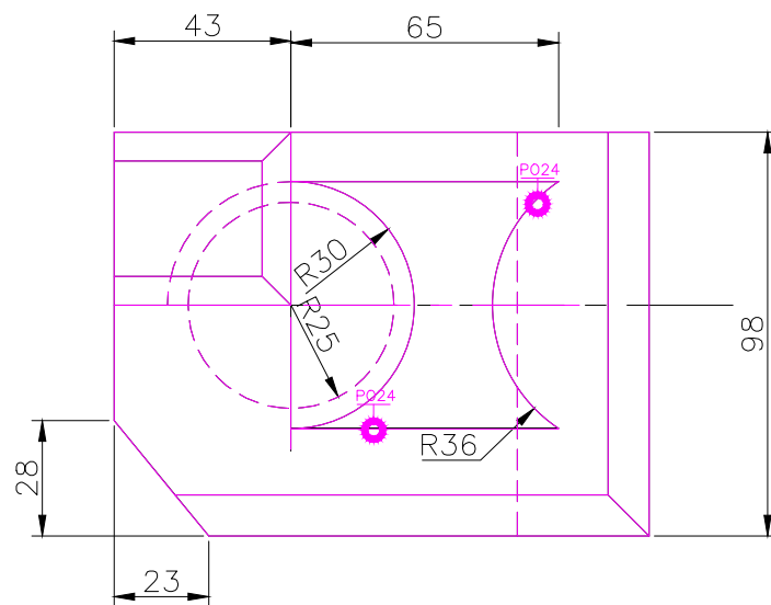
TOP SCALE 1/2
