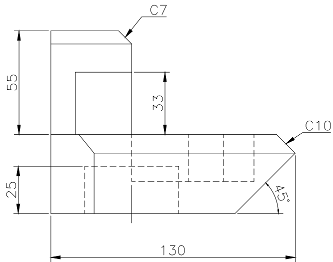
FRONT SCALE 1/2
