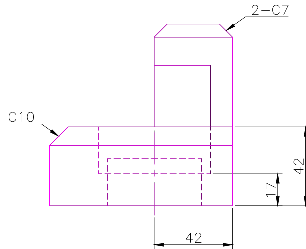
RIGHT SCALE 1/2
