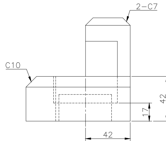
RIGHT SCALE 1/2
