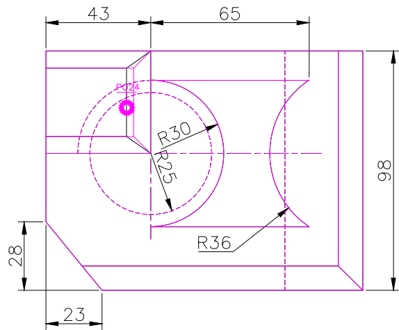
TOP SCALE 1/2
