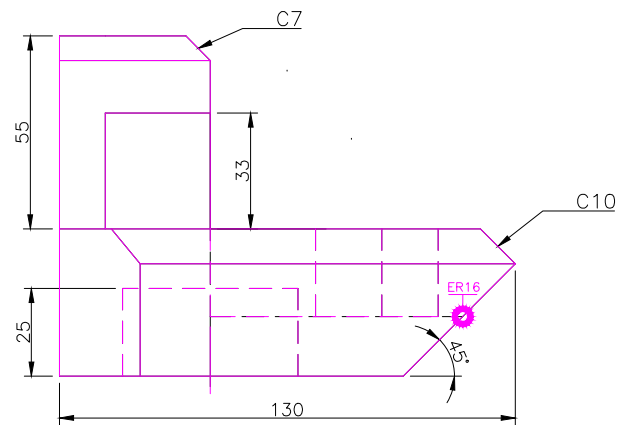
FRONT SCALE 1/2
