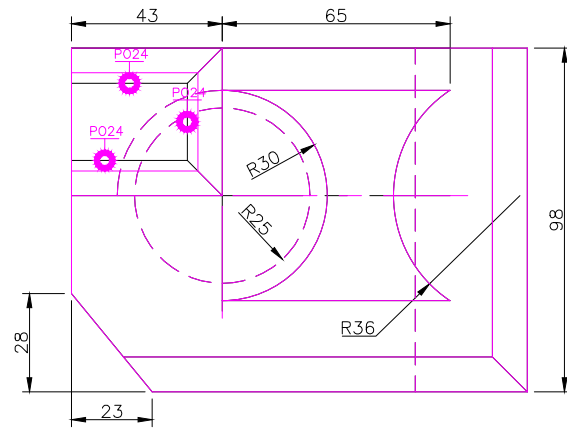
TOP SCALE 1/2
