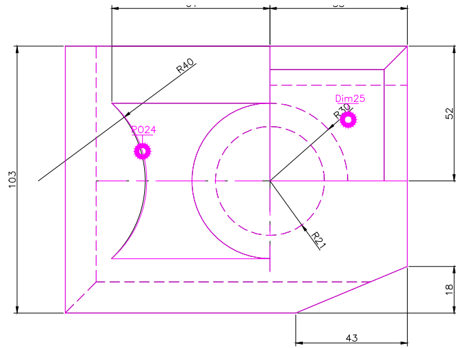
TOP SCALE 1/2
