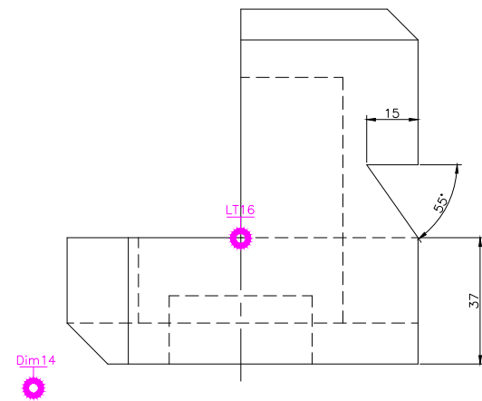
RIGHT SCALE 1/2
