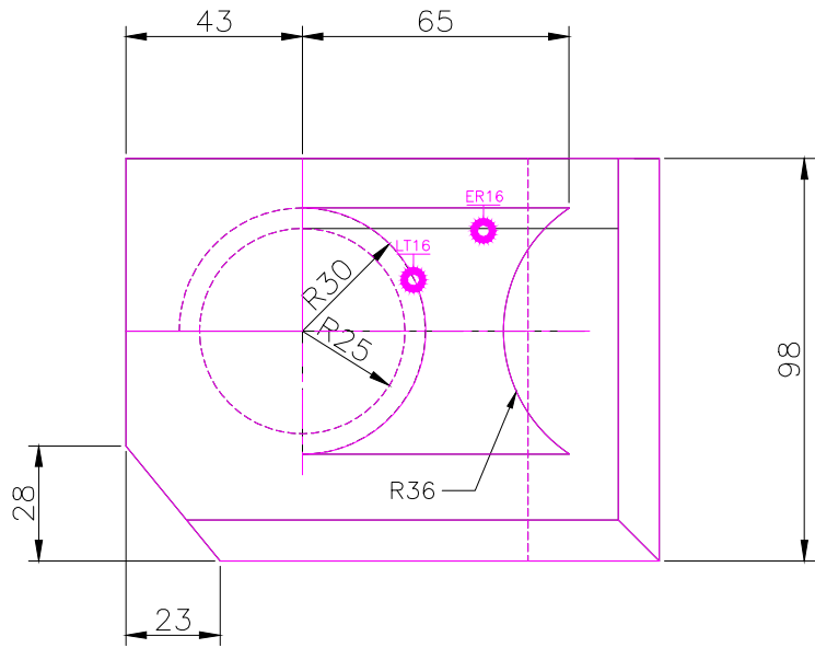
TOP SCALE 1/2
