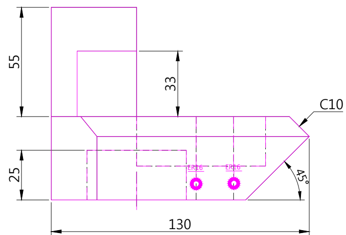
FRONT scale 1/2
