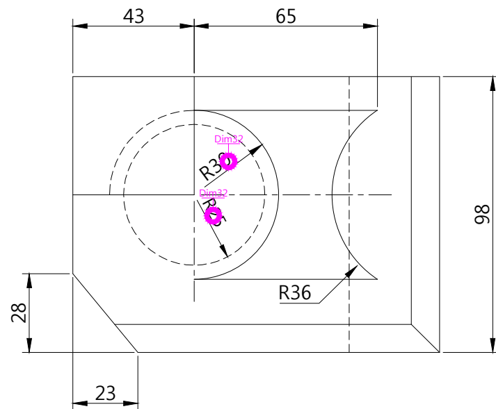
TOP scale 1/2
