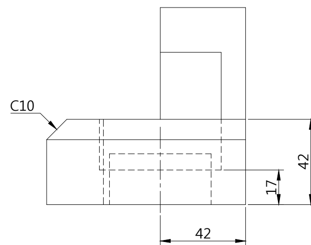
RIGHT scale 1/2
