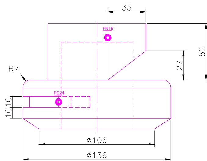
FRONT SCALE 1/2
