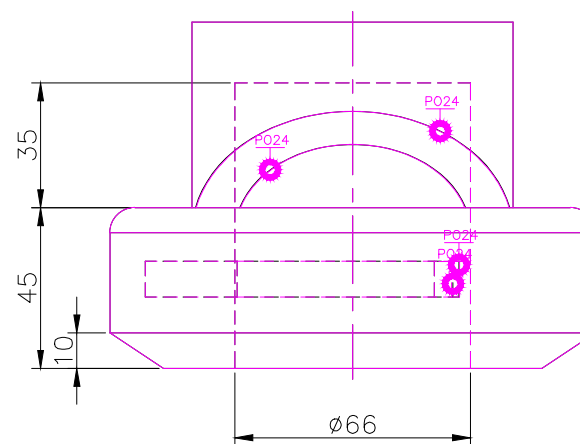
RIGHT SCALE 1/2
