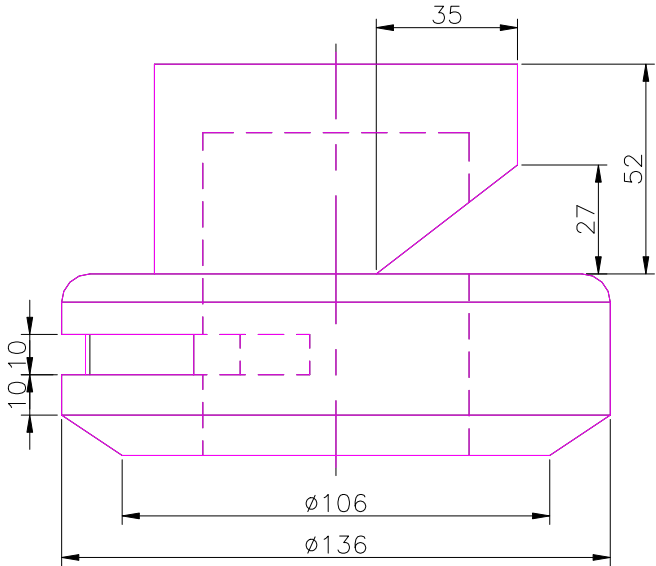
FRONT SCALE 1/2
