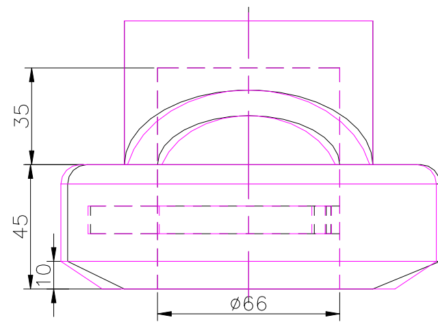
RIGHT SCALE 1/2
