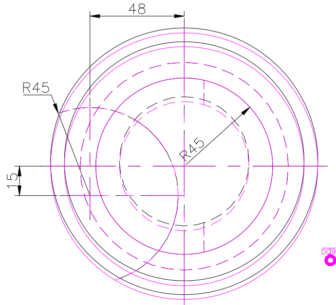
TOP SCALE 1/2
