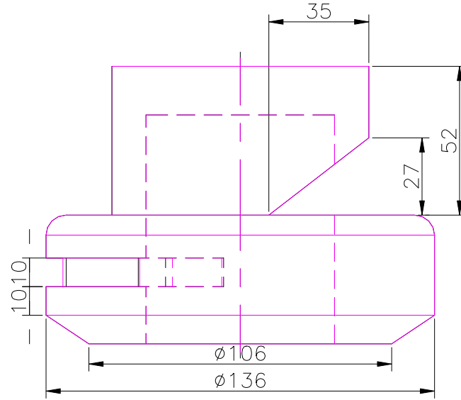
FRONT SCALE 1/2
