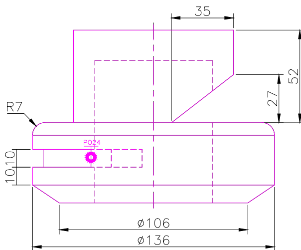
FRONT SCALE 1/2
