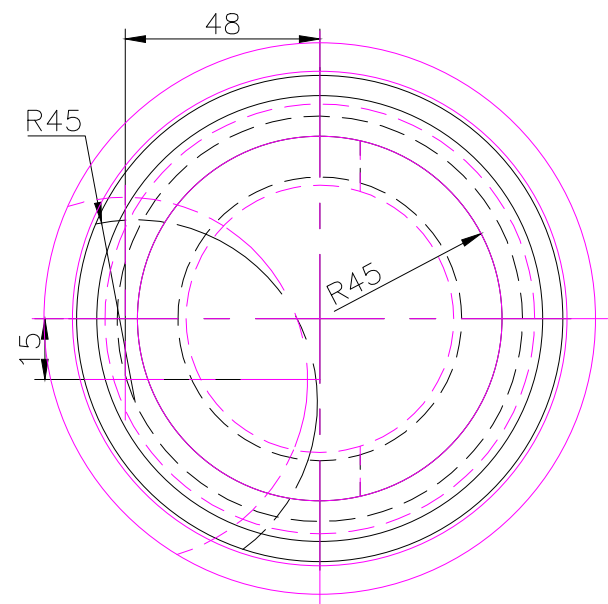
TOP SCALE 1/2
