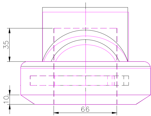
RIGHT SCALE 1/2
