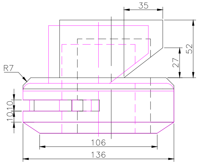
FRONT SCALE 1/2
