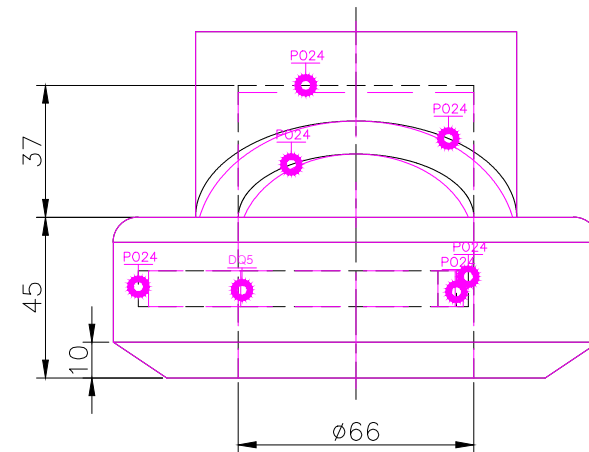
RIGHT SCALE 1/2
