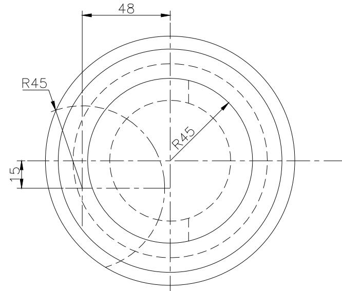
TOP SCALE 1/2
