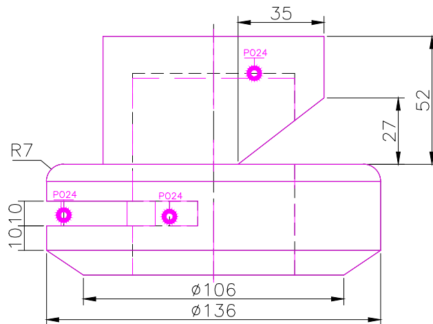
FRONT SCALE 1/2
