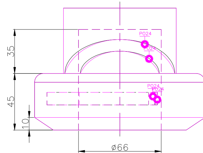
RIGHT SCALE 1/2
