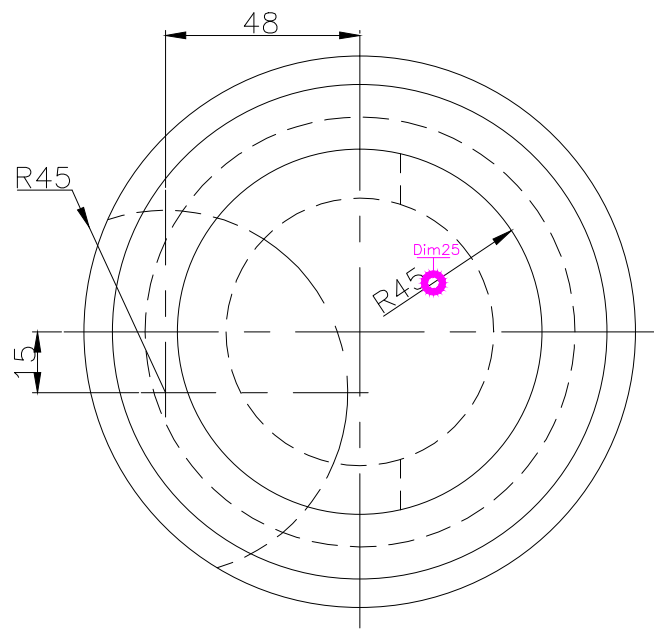
TOP SCALE 1/2
