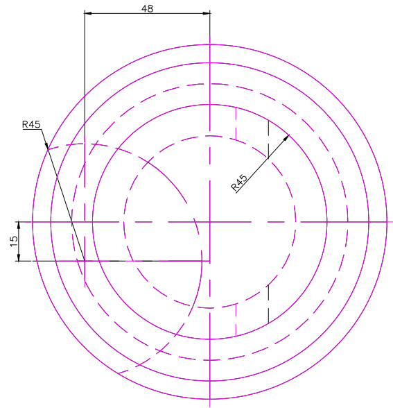
TOP SCALE 1/2
