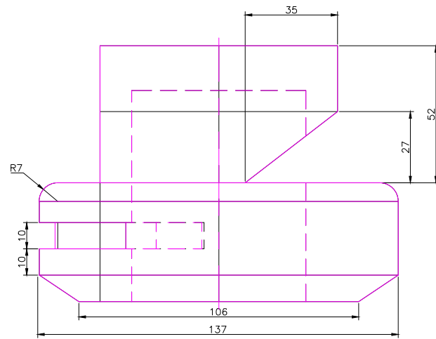
FRONT SCALE 1/2
