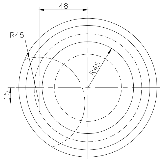
TOP SCALE 1/2
