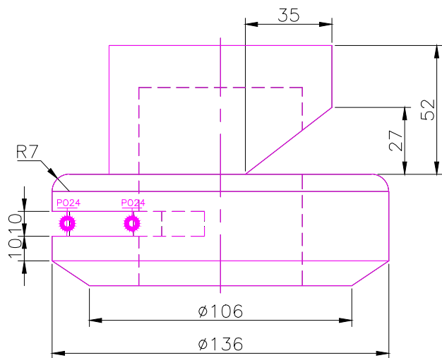
FRONT SCALE 1/2
