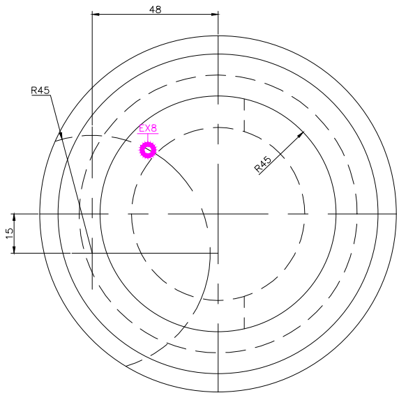
TOP SCALE 1/2
