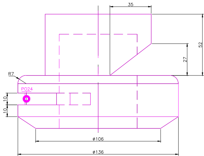
FRONT SCALE 1/2
