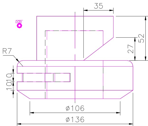
FRONT SCALE 1/2
